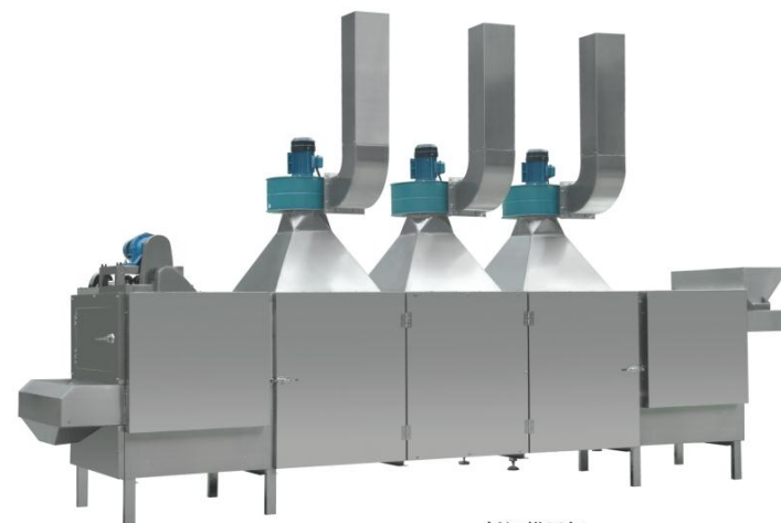
ZHKX-III-L 低温烘干机 Low Temperature Dryer
